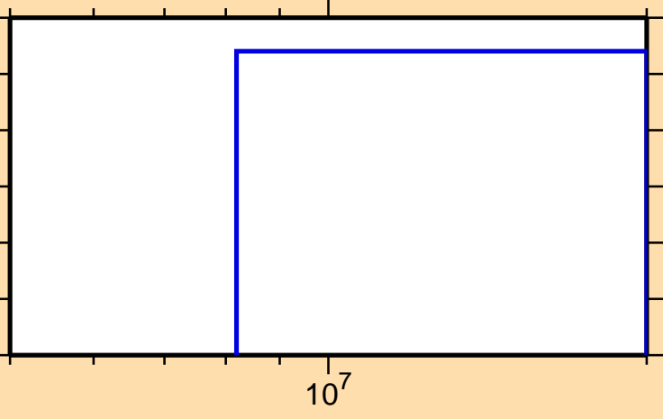
\sigma vs. E for ^{161}\text{Ho}(n,t)
