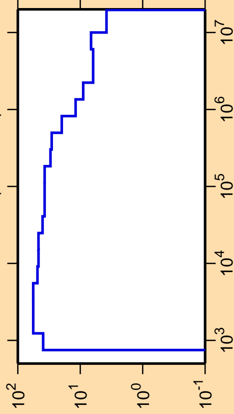
\Delta\sigma/\sigma vs. E for ^{161}\text{Ho}(n,\text{nonel.})
