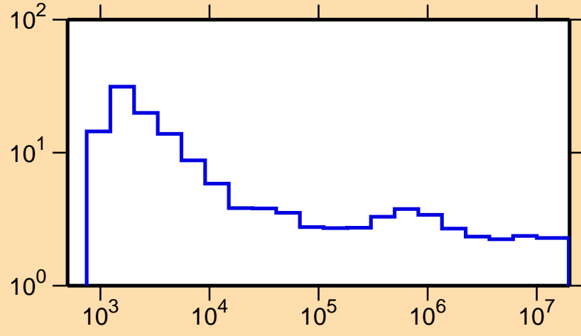
\sigma vs. E for ^{161}\text{Ho}(n,\text{nonel.})
