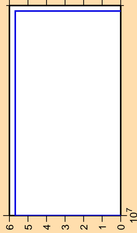
\Delta\sigma/\sigma vs. E for ^{161}\text{Ho}(\text{mt117})
