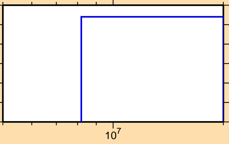
\sigma vs. E for ^{161}\text{Ho}(n,3n)
