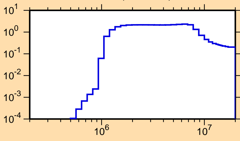
\sigma vs. E for ^{162}\text{Ho}(n,n\text{cont.})
