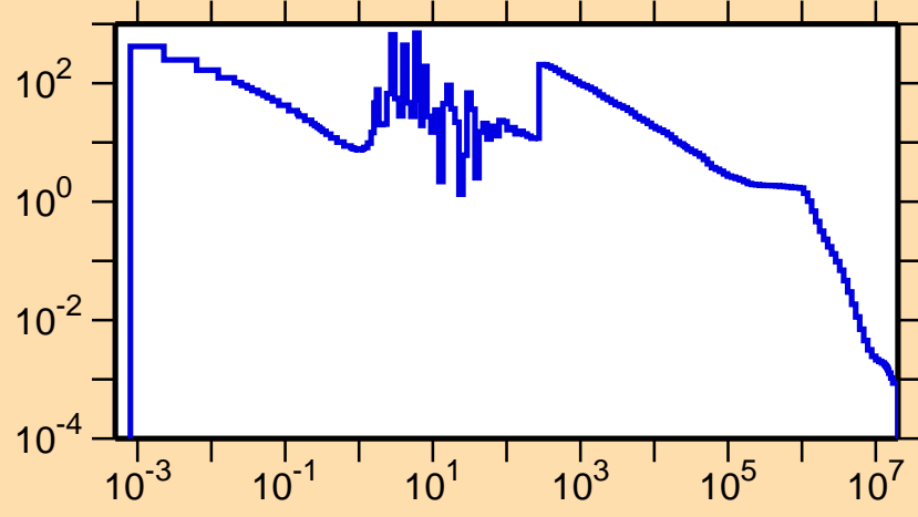
\sigma vs. E for ^{162}\text{Ho}(n,\gamma)
