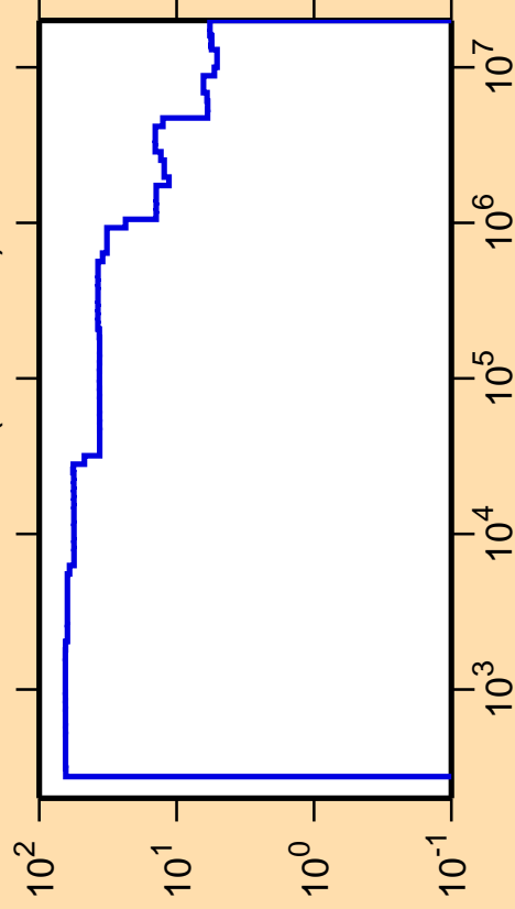
\Delta\sigma/\sigma vs. E for ^{162}\text{Ho}(n,\text{nonel.})
