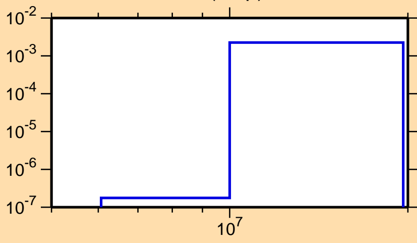
\sigma vs. E for ^{162}\text{Ho}(n,np)
