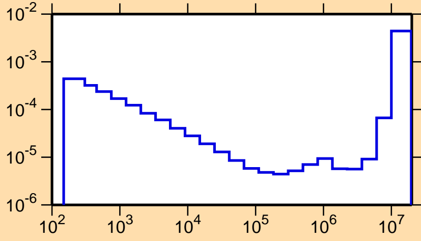
\sigma vs. E for ^{162}\text{Ho}(n,\alpha)
