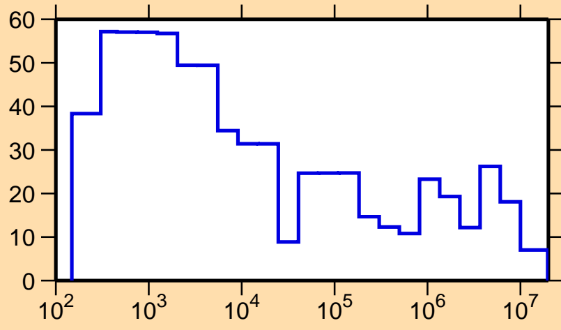
\Delta\sigma/\sigma vs. E for ^{162}\text{Ho}(n,\text{el.})
