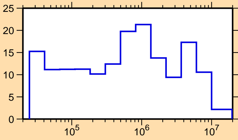
\Delta\sigma/\sigma vs. E for ^{162}\text{Ho}(n,\text{tot.})
