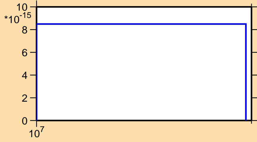
\sigma vs. E for ^{162}\text{Ho} (mt 45)
