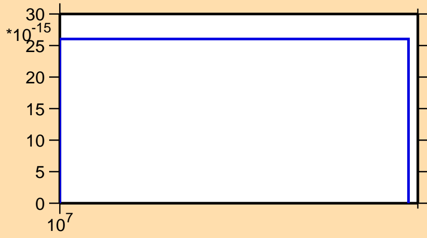
\sigma vs. E for ^{162}\text{Ho}(\text{mt117})
