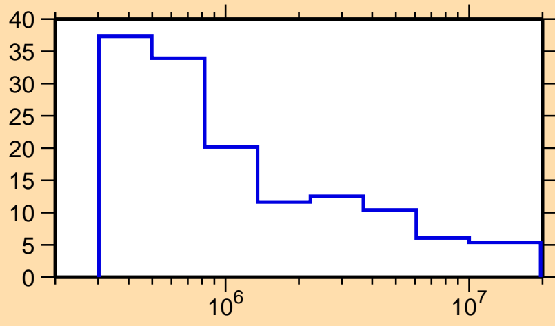
\Delta\sigma/\sigma vs. E for ^{162}\text{Ho}(n,\text{nonel.})
