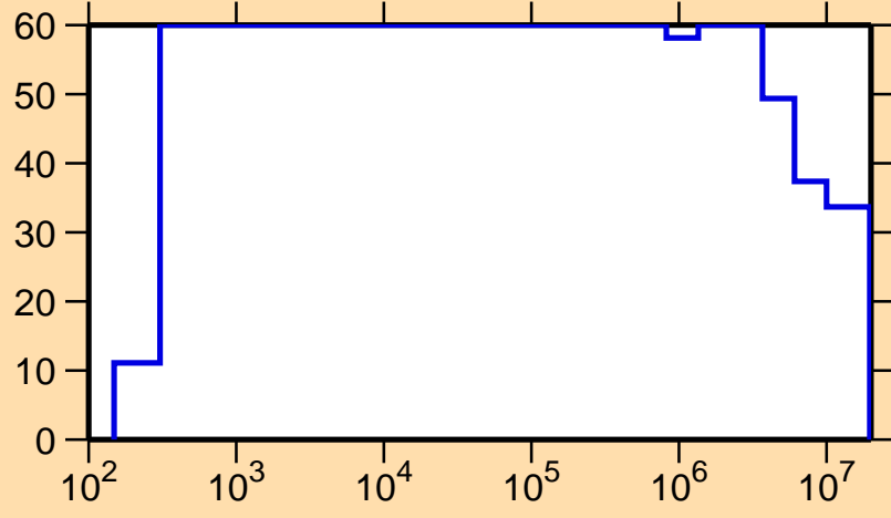
\Delta\sigma/\sigma vs. E for ^{162}\text{Ho}(n,p)
