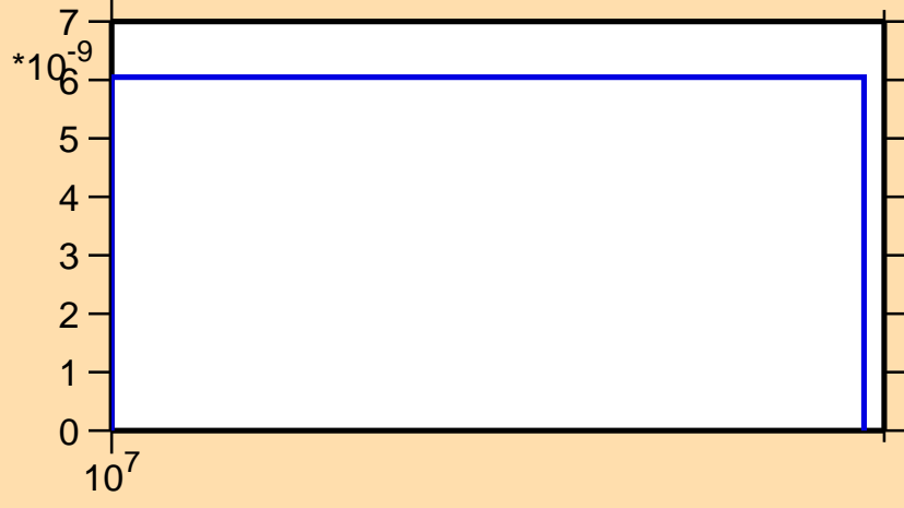
\sigma vs. E for ^{162}\text{Ho}(n,nt)
