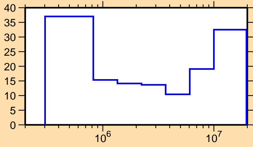
\Delta\sigma/\sigma vs. E for ^{162}\text{Ho}(n,n\text{cont.})
