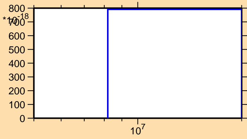
\sigma vs. E for ^{162}\text{Ho} (mt 34)
