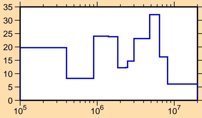
\Delta\sigma/\sigma vs. E for ^{162}\text{Ho}(n, el.)
