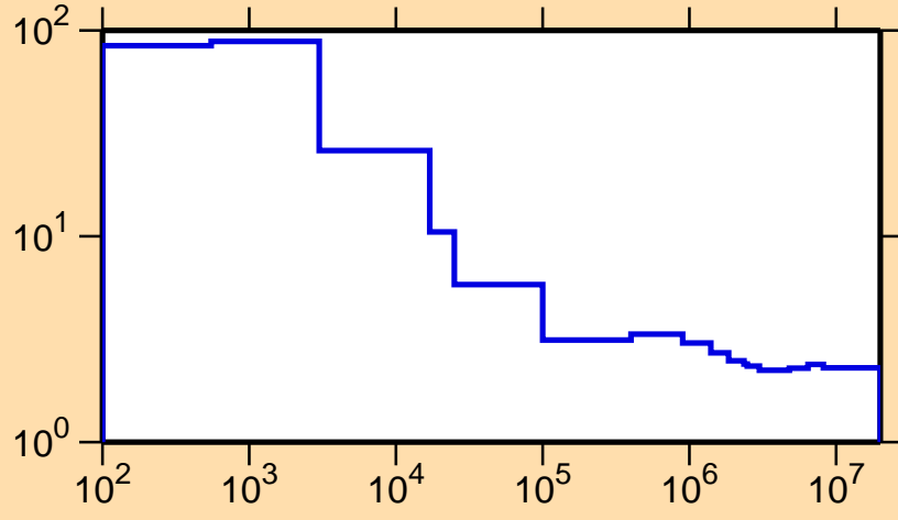
\sigma vs. E for ^{162}\text{Ho}(n,\text{nonel.})
