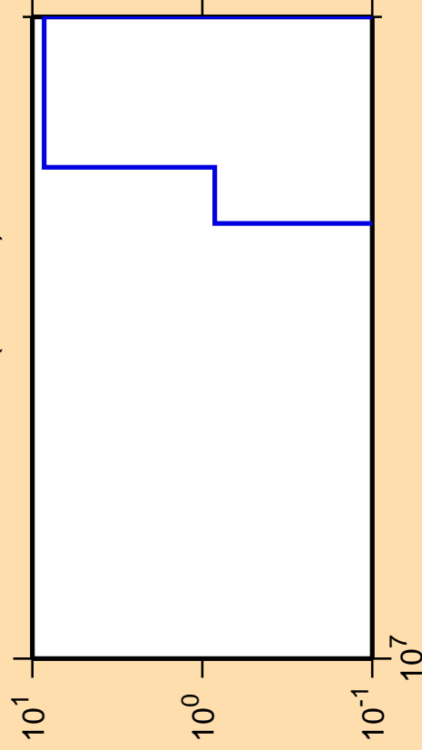
\Delta\sigma/\sigma vs. E for ^{162}\text{Ho}(\text{mt117})
