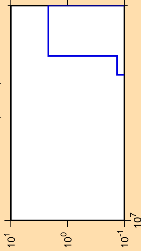
\Delta\sigma/\sigma vs. E for ^{162}\text{Ho} (mt 45)
