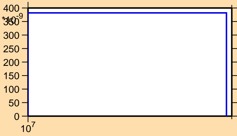
\sigma vs. E for ^{162}\text{Ho}(n,2np)
