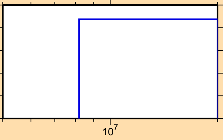
\sigma vs. E for ^{162}\text{Ho} (mt 45)
