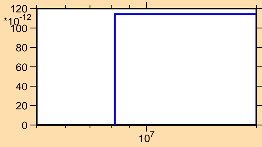
\sigma vs. E for ^{162}\text{Ho}(n,p\alpha)
