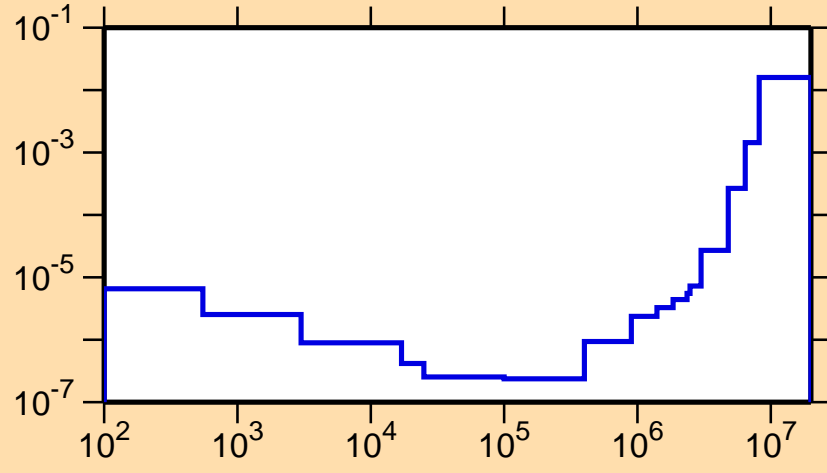
\sigma vs. E for ^{162}\text{Ho}(n,p)
