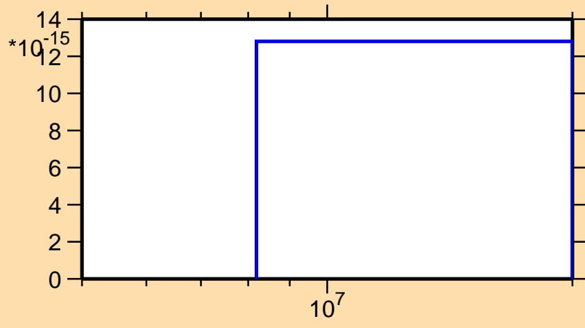
\sigma vs. E for ^{162}\text{Ho}(\text{mt117})
