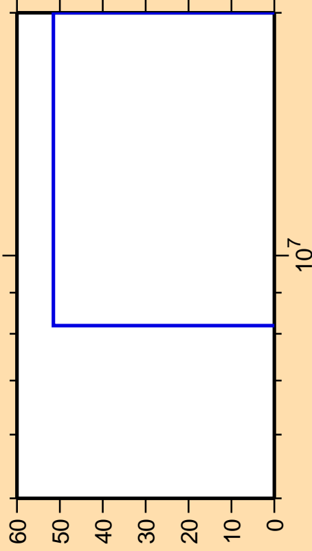
\Delta\sigma/\sigma vs. E for ^{162}\text{Ho}(n,3n)
