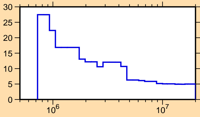
\Delta\sigma/\sigma vs. E for ^{163}\text{Ho}(n,n\text{onel.})
