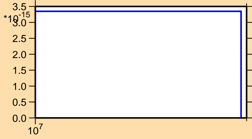
\sigma vs. E for ^{163}\text{Ho} (mt 45)
