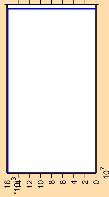
\Delta\sigma/\sigma vs. E for ^{163}\text{Ho} (mt 45)
