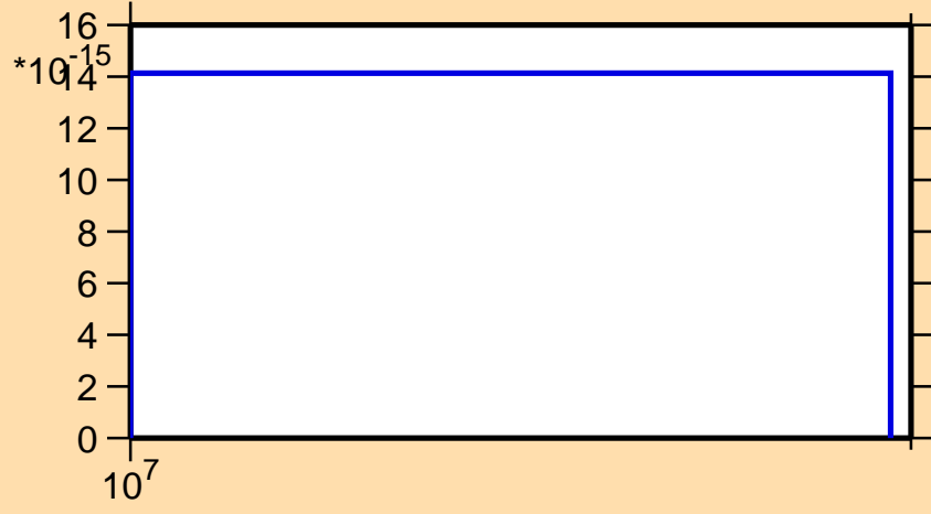
\sigma vs. E for ^{163}\text{Ho}(\text{mt117})
