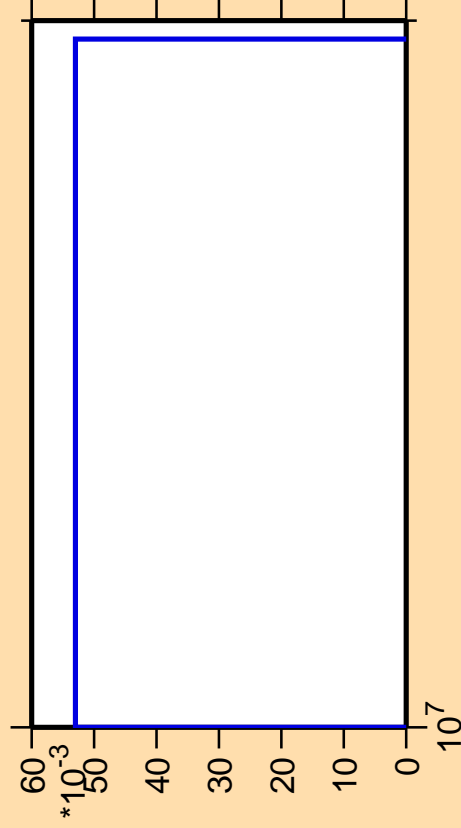
\Delta\sigma/\sigma vs. E for ^{163}\text{Ho}(\text{mt117})
