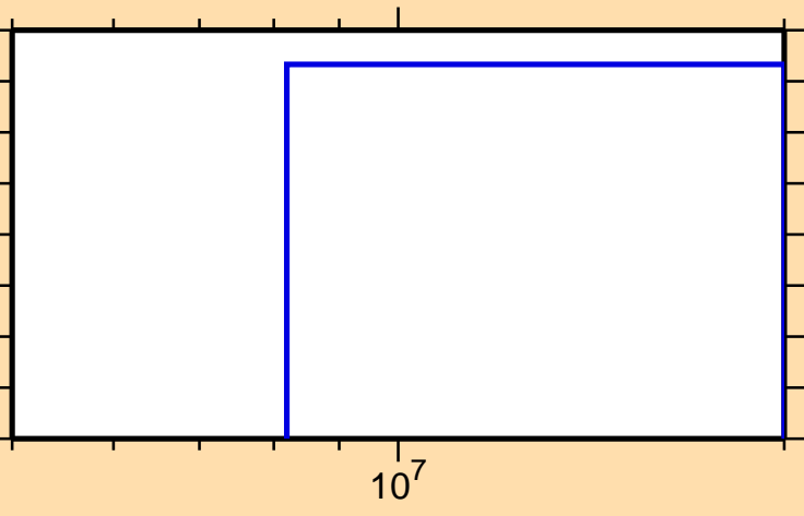
\sigma vs. E for ^{163}\text{Ho}(n,2np)
