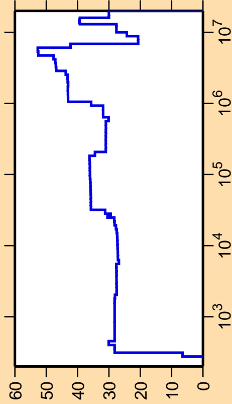
\Delta\sigma/\sigma vs. E for ^{163}\text{Ho}(n,\gamma)
