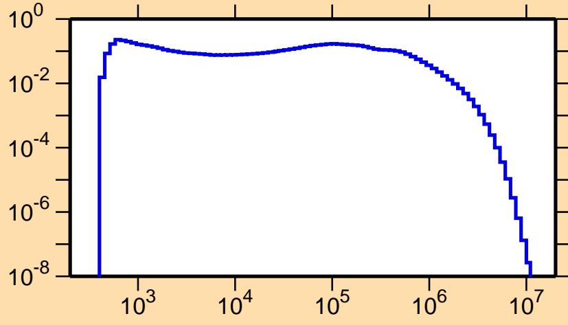
\sigma vs. E for ^{163}\text{Ho}(n,n_1)
