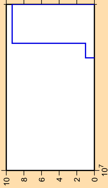
\Delta\sigma/\sigma vs. E for ^{163}\text{Ho}(\text{mt117})
