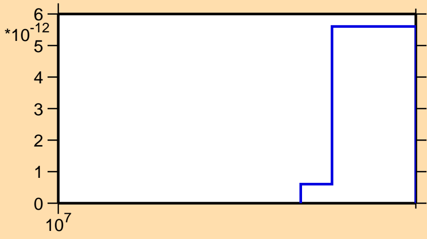
\sigma vs. E for ^{163}\text{Ho}(\text{mt117})
