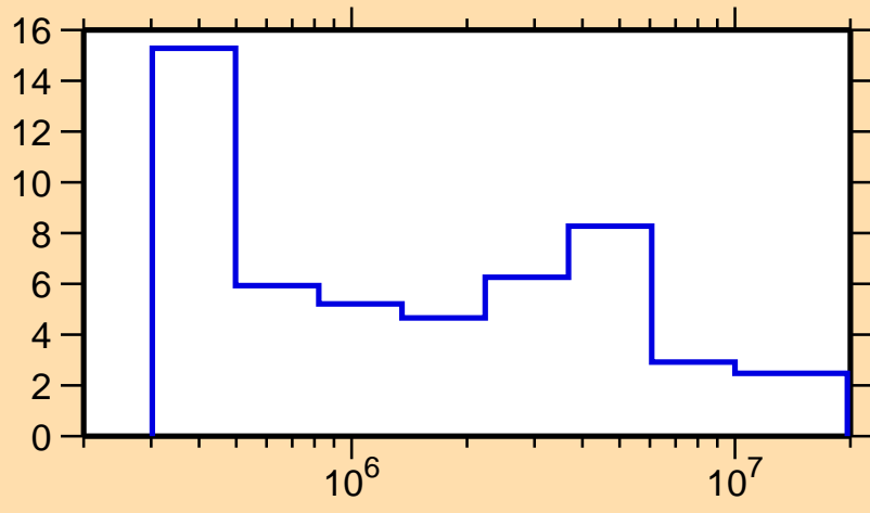
\Delta\sigma/\sigma vs. E for ^{163}\text{Ho}(n, el.)
