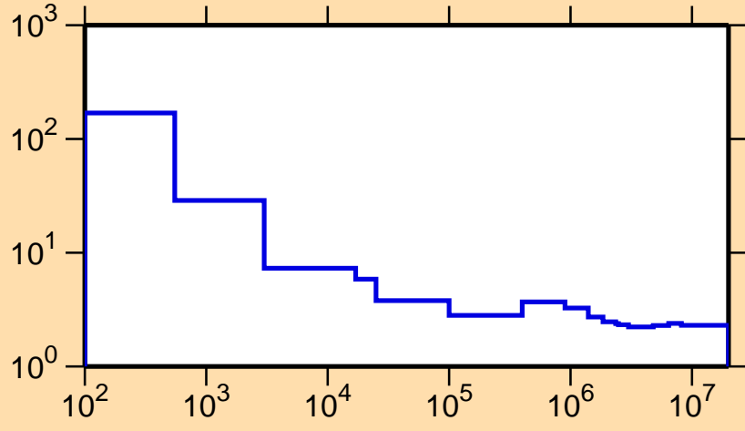
\sigma vs. E for ^{163}\text{Ho}(n,\text{nonel.})
