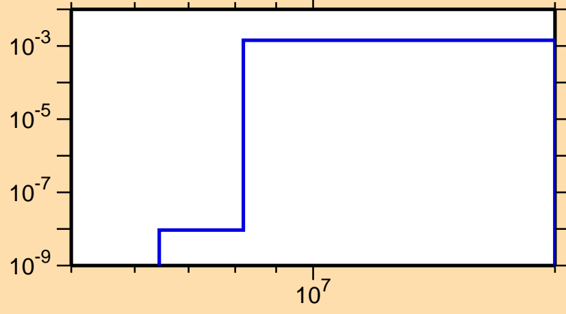
\sigma vs. E for ^{163}\text{Ho}(n,np)
