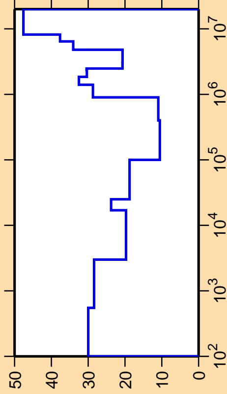
\Delta\sigma/\sigma vs. E for ^{163}\text{Ho}(n,n_2)
