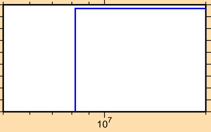
\sigma vs. E for ^{163}\text{Ho}(n,nt)
