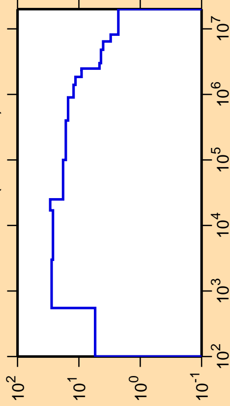
\Delta\sigma/\sigma vs. E for ^{163}\text{Ho}(n,\text{nonel.})
