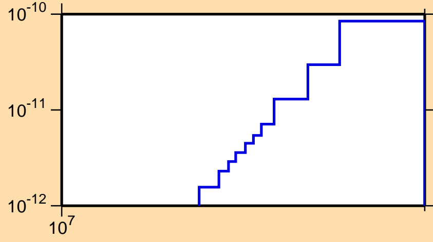
\sigma vs. E for ^{164}\text{Ho}(n,p\alpha)
