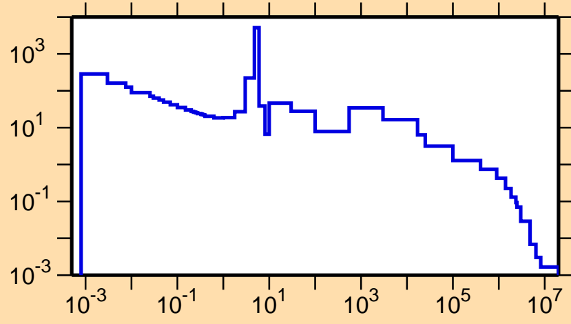
\sigma vs. E for ^{164}\text{Ho}(n,\gamma)
