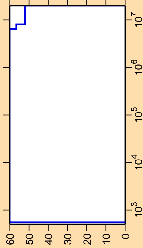
\Delta\sigma/\sigma vs. E for ^{164}\text{Ho}(n,p)
