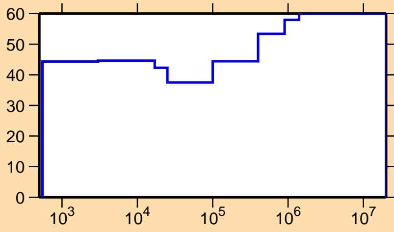
\Delta\sigma/\sigma vs. E for ^{164}\text{Ho}(n,\gamma)
