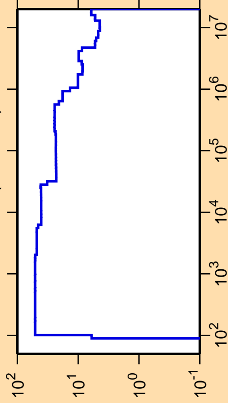
\Delta\sigma/\sigma vs. E for ^{164}\text{Ho}(n,\text{nonel.})
