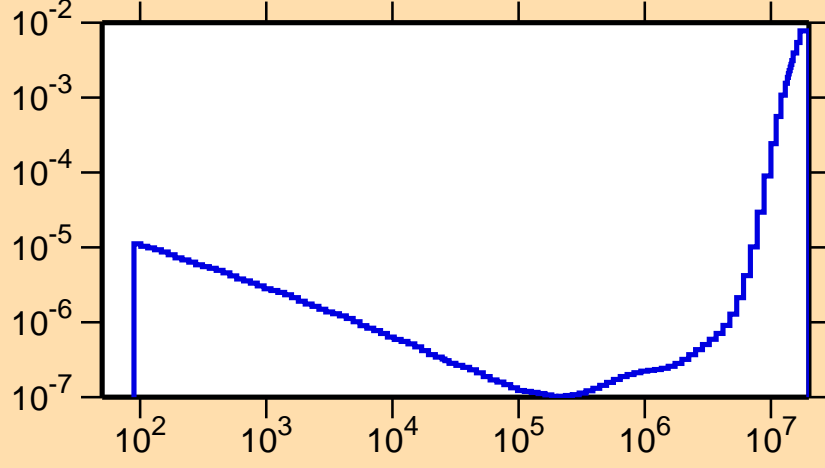
\sigma vs. E for ^{164}\text{Ho}(n,\alpha)
