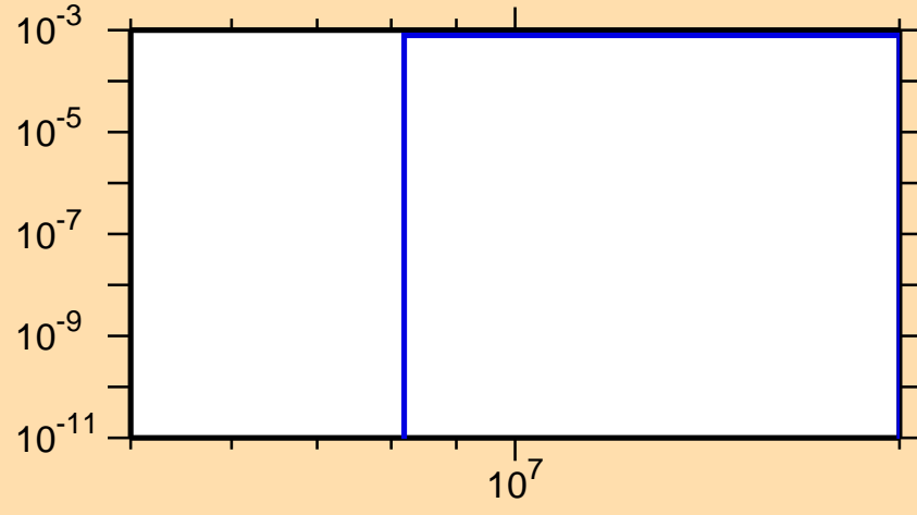
\sigma vs. E for ^{164}\text{Ho}(n,np)
