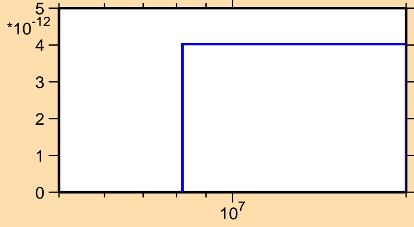
\sigma vs. E for ^{164}\text{Ho}(n,p\alpha)
