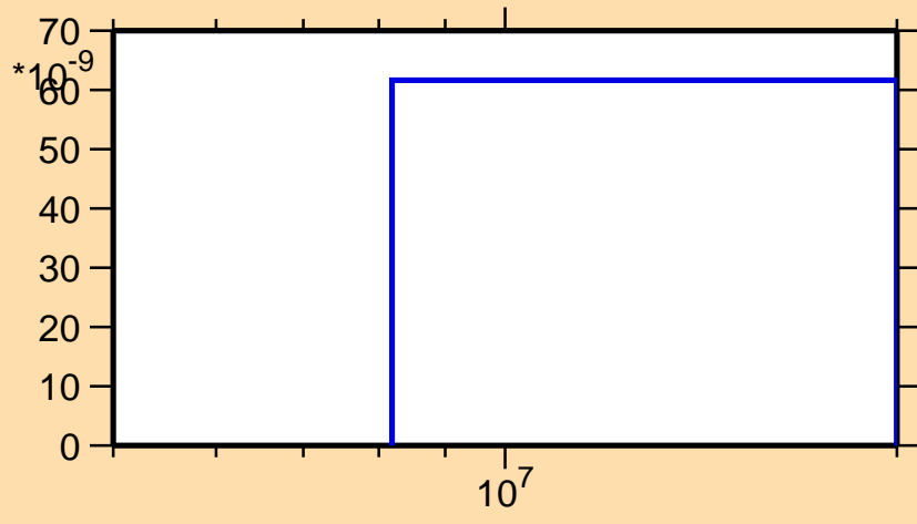
\sigma vs. E for ^{164}\text{Ho}(n,2np)
