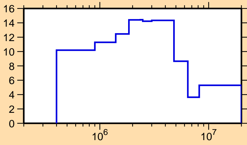
\Delta\sigma/\sigma vs. E for ^{164}\text{Ho}(n,\text{el.})
