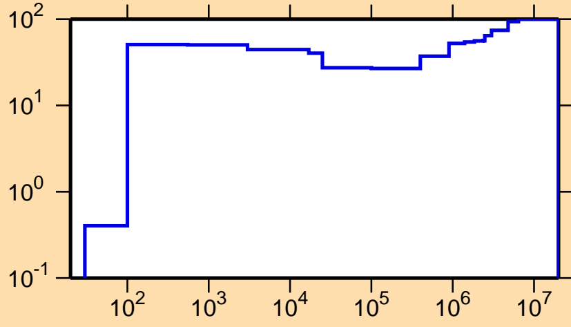
\Delta\sigma/\sigma vs. E for ^{164}\text{Ho}(n,\gamma)
