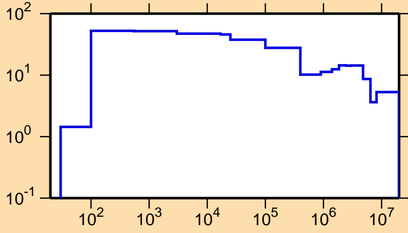
\Delta\sigma/\sigma vs. E for ^{164}\text{Ho}(n,\text{el.})
