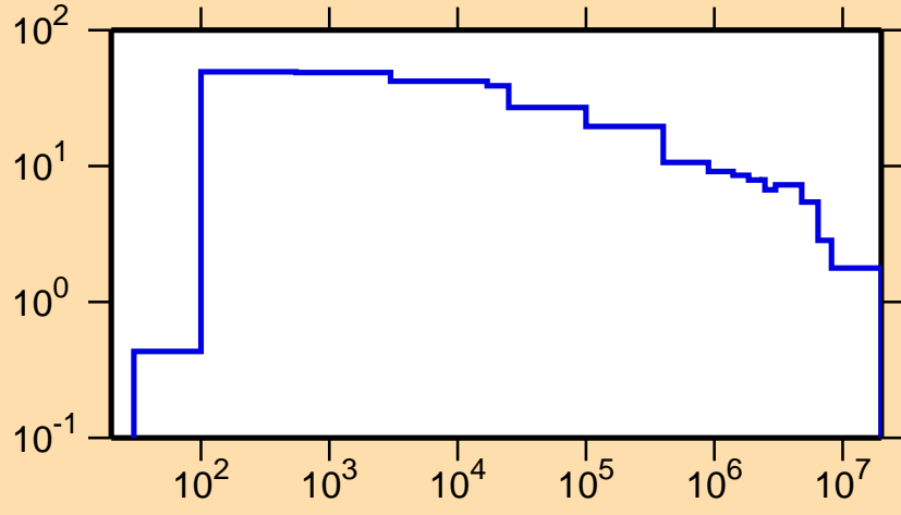
\Delta\sigma/\sigma vs. E for ^{164}\text{Ho}(n,\text{tot.})
