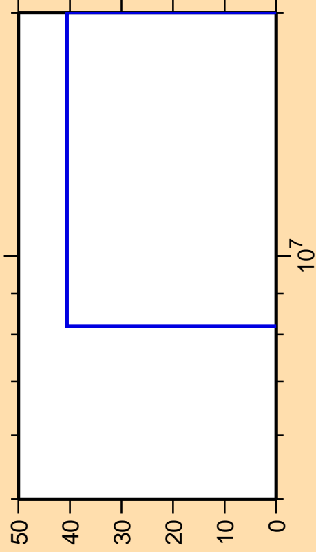
\Delta\sigma/\sigma vs. E for ^{164}\text{Ho}(n,3n)
