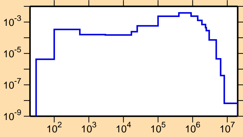
\sigma vs. E for ^{164}\text{Ho}(n,n_2)
