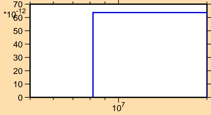
\sigma vs. E for ^{164}\text{Ho}(n,\text{He3})
