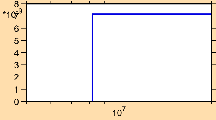
\sigma vs. E for ^{164}\text{Ho}(n,nt)
