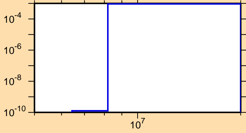
\sigma vs. E for ^{164}\text{Ho}(n,d)
