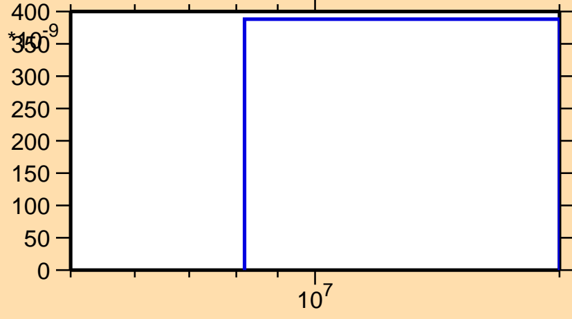
\sigma vs. E for ^{164}\text{Ho}(n,\text{nd})
