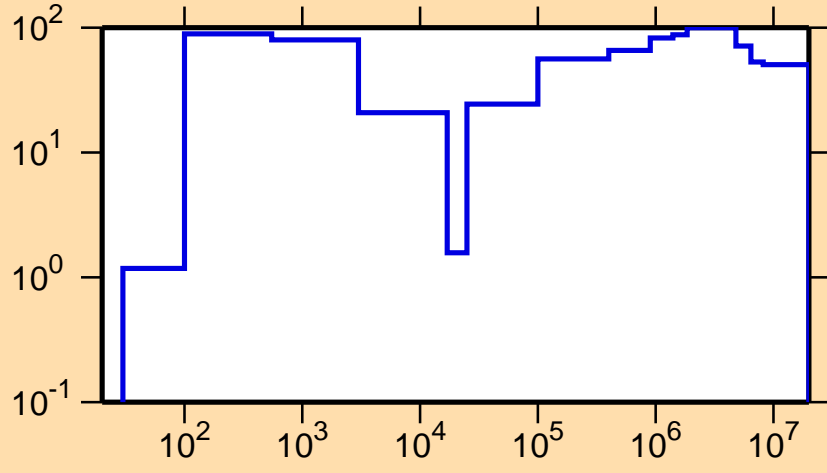
\Delta\sigma/\sigma vs. E for ^{164}\text{Ho}(n,p)
