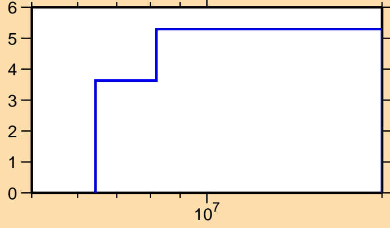
\Delta\sigma/\sigma vs. E for ^{164}\text{Ho}(n,\text{el.})
