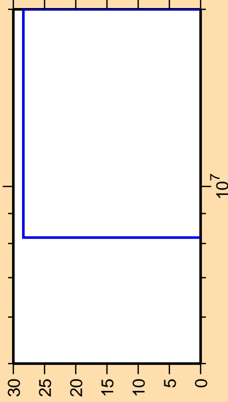
\Delta\sigma/\sigma vs. E for ^{164}\text{Ho}(n,p\alpha)
