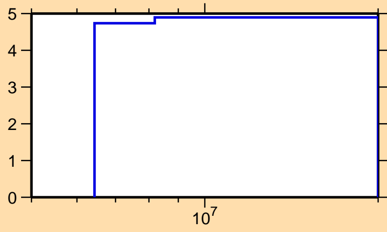
\Delta\sigma/\sigma vs. E for ^{164}\text{Ho}(n,\text{nonel.})
