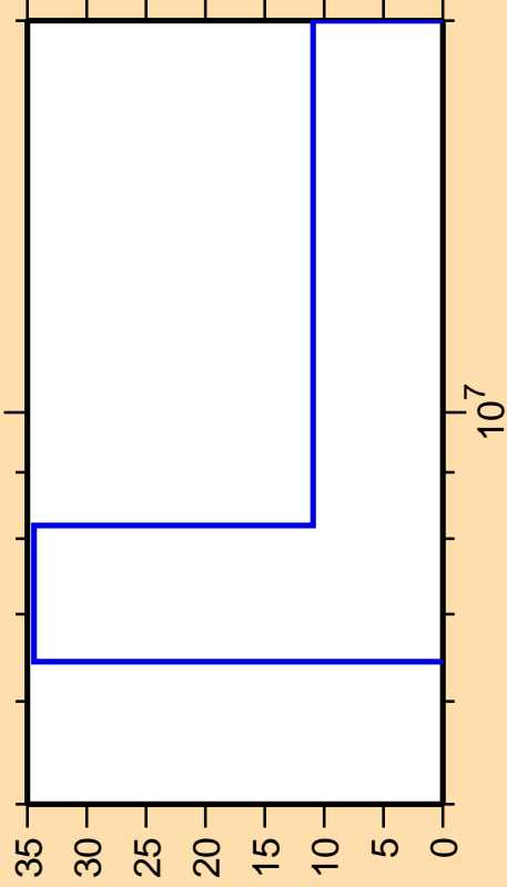
\Delta\sigma/\sigma vs. E for ^{164}\text{Ho}(n,2n)
