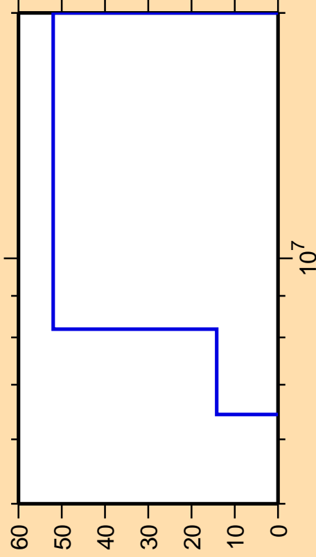
\Delta\sigma/\sigma vs. E for ^{164}\text{Ho}(n,np)
