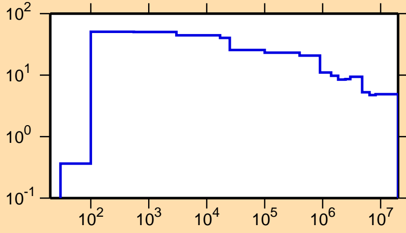
\Delta\sigma/\sigma vs. E for ^{164}\text{Ho}(n,\text{nonel.})
