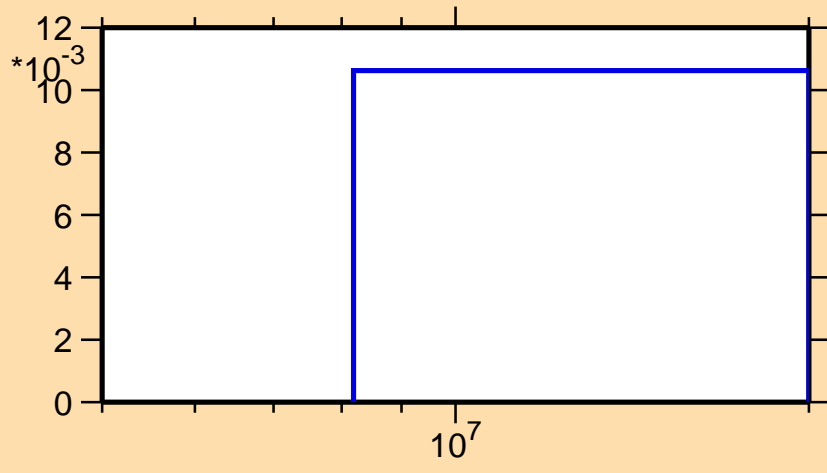
\sigma vs. E for ^{164}\text{Ho}(n,3n)
