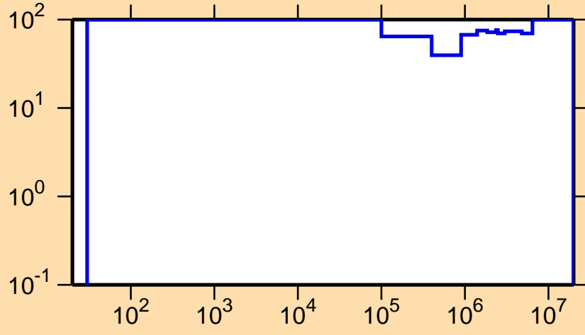
\Delta\sigma/\sigma vs. E for ^{164}\text{Ho}(n,n_1)
