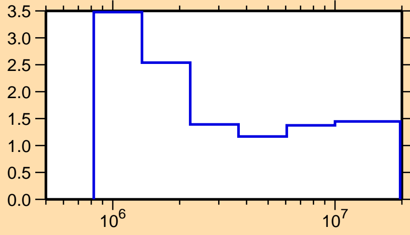
\Delta\sigma/\sigma vs. E for ^{165}\text{Ho}(n,n\text{nonel.})
