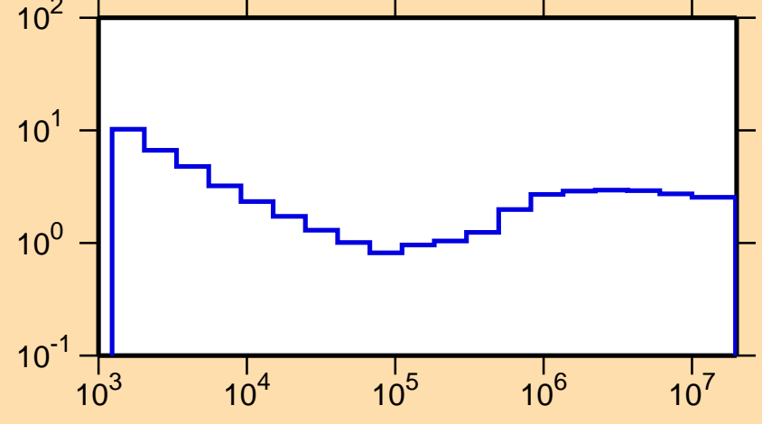
\sigma vs. E for ^{165}\text{Ho}(n,\text{nonel.})
