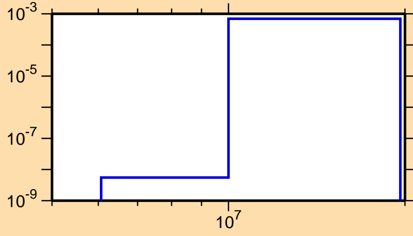
\sigma vs. E for ^{165}\text{Ho}(n,d)
