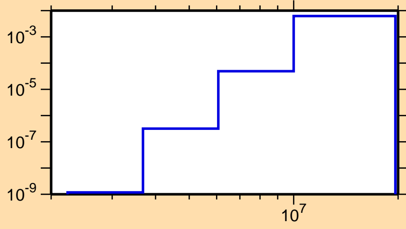
\sigma vs. E for ^{165}\text{Ho}(n,p)
