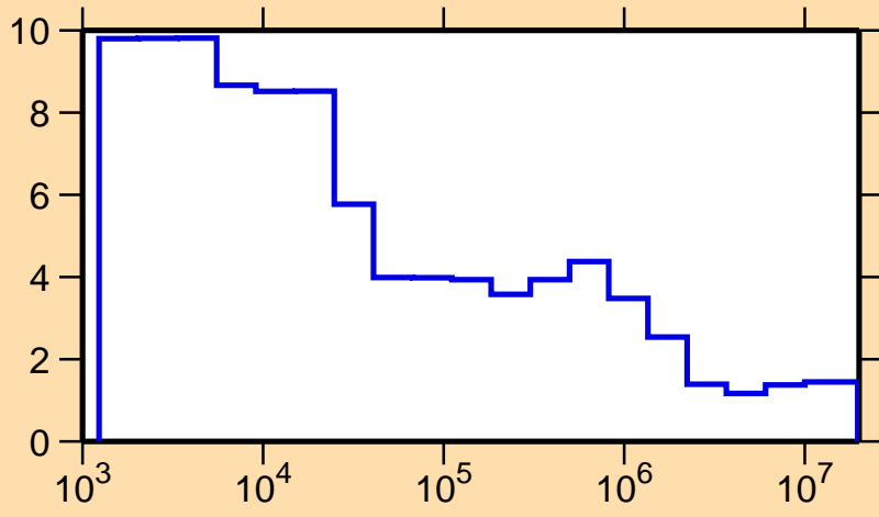
\Delta\sigma/\sigma vs. E for ^{165}\text{Ho}(n,\text{nonel.})
