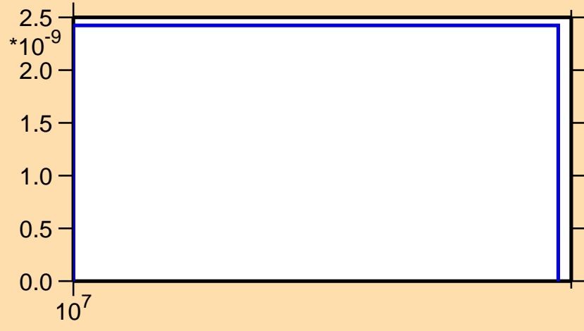
\sigma vs. E for ^{165}\text{Ho}(n,2n\alpha)
