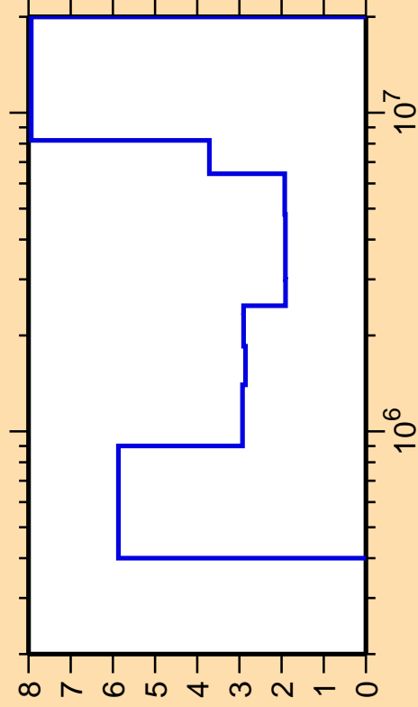
\Delta\sigma/\sigma vs. E for ^{165}\text{Ho}(n,n\text{cont.})
