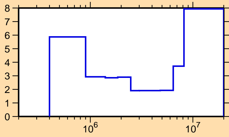
\Delta\sigma/\sigma vs. E for ^{165}\text{Ho}(n,n\text{cont.})
