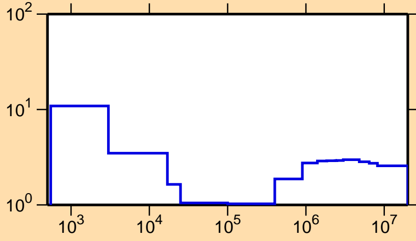
\sigma vs. E for ^{165}\text{Ho}(n,\text{nonel.})
