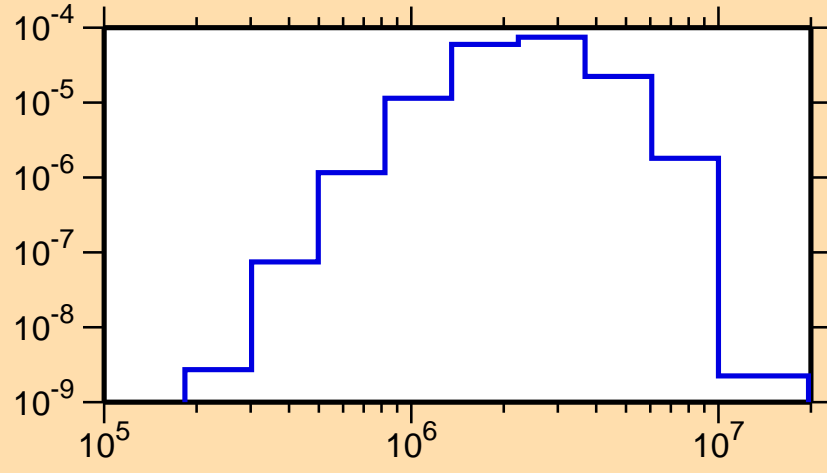
\sigma vs. E for ^{166}\text{Ho}(n,n_4)
