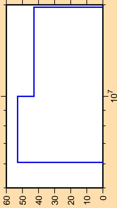
\Delta\sigma/\sigma vs. E for ^{166}\text{Ho}(n,np)
