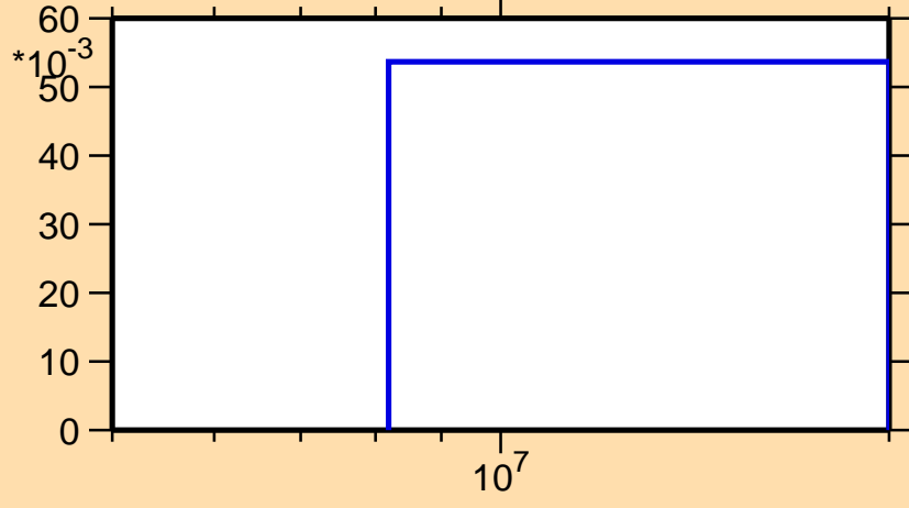
\sigma vs. E for ^{166}\text{Ho}(n,3n)
