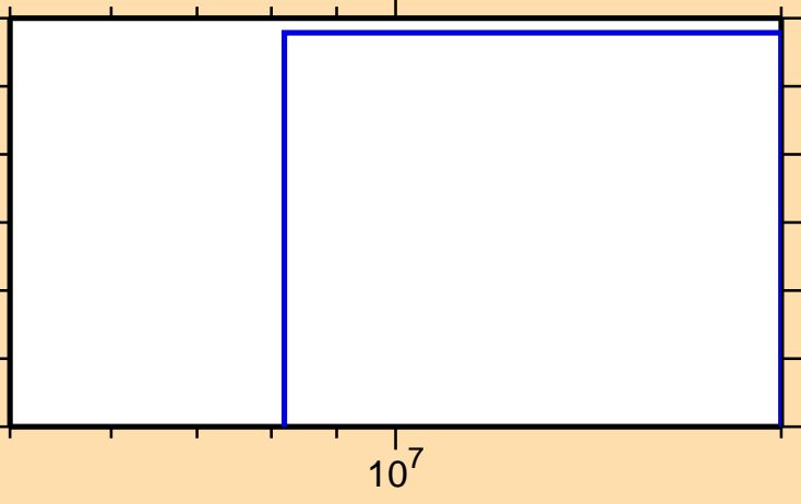
\sigma vs. E for ^{166}\text{Ho}(n,2n\alpha)
