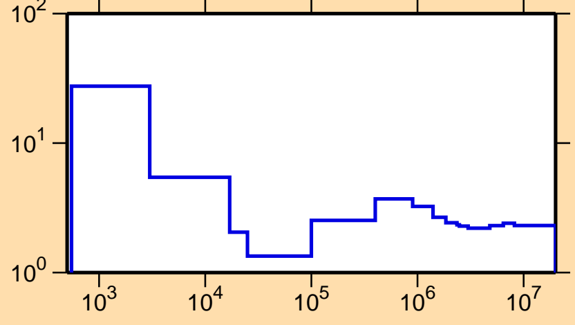
\sigma vs. E for ^{166}\text{Ho}(n,\text{nonel.})
