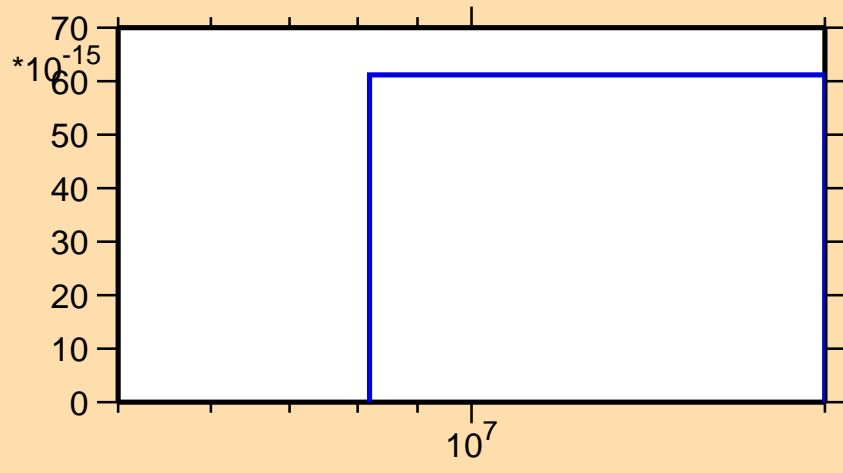
\sigma vs. E for ^{166}\text{Ho}(n,p\alpha)
