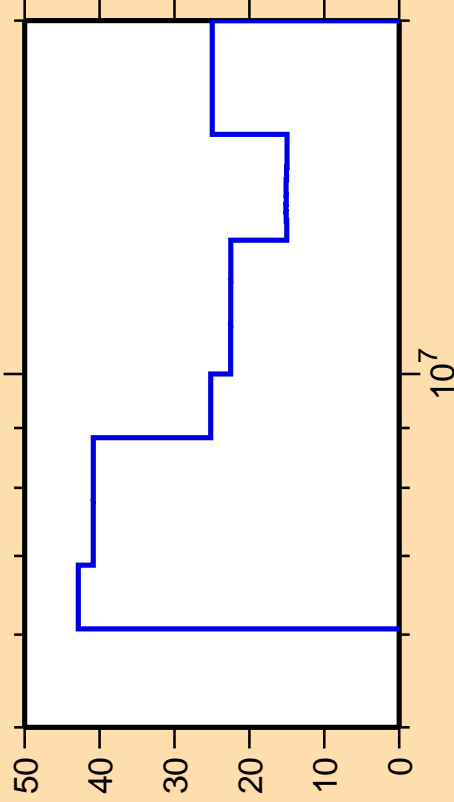
\Delta\sigma/\sigma vs. E for ^{166}\text{Ho}(n,2n)
