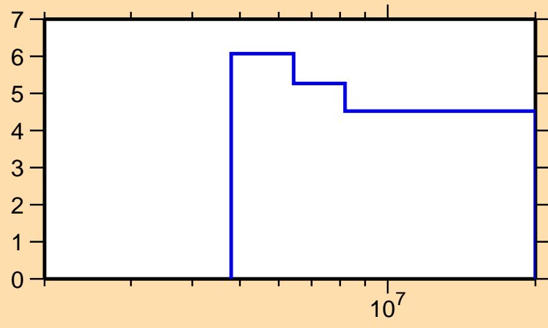
\Delta\sigma/\sigma vs. E for ^{166}\text{Ho}(n,\text{nonel.})
