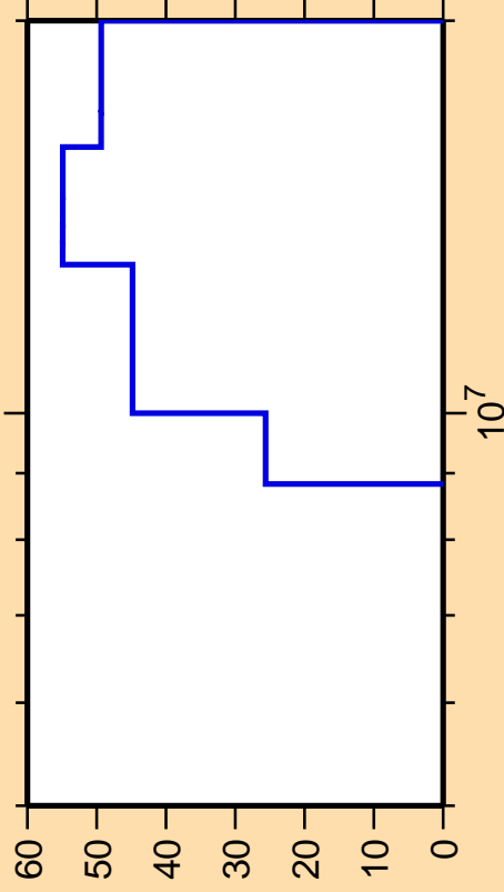
\Delta\sigma/\sigma vs. E for ^{167}\text{Ho}(n,np)
