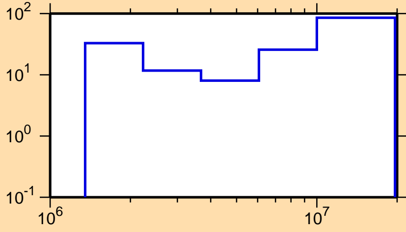
\Delta\sigma/\sigma vs. E for ^{167}\text{Ho}(n,n\text{cont.})
