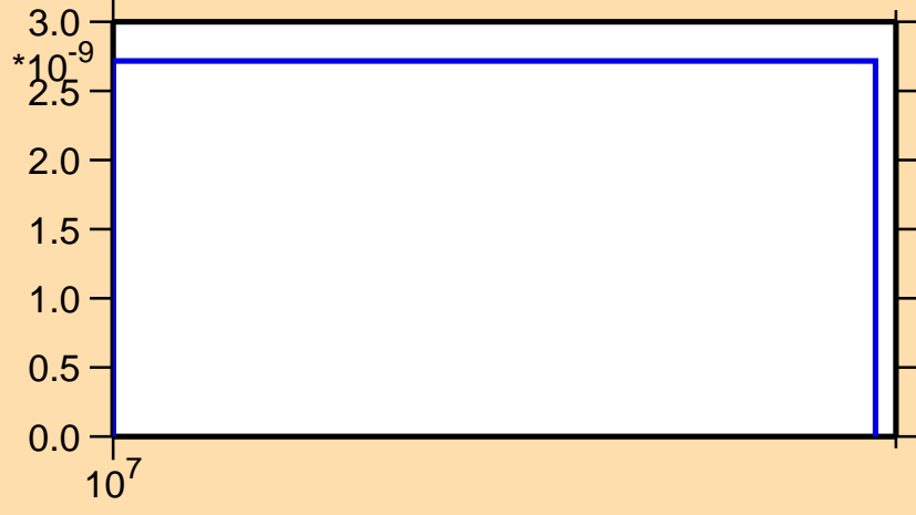
\sigma vs. E for ^{167}\text{Ho}(n,2n\alpha)
