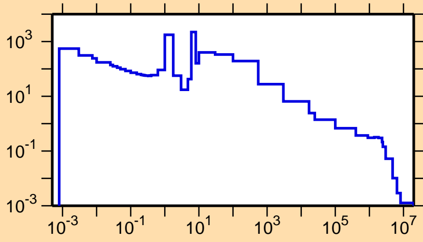
\sigma vs. E for ^{167}\text{Ho}(n,\gamma)
