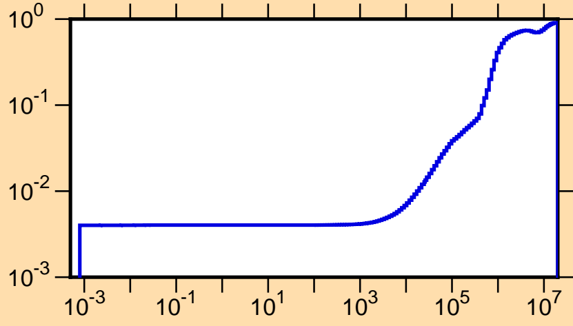
\mu vs. E for ^{168}\text{Ho}(\text{mt251})
