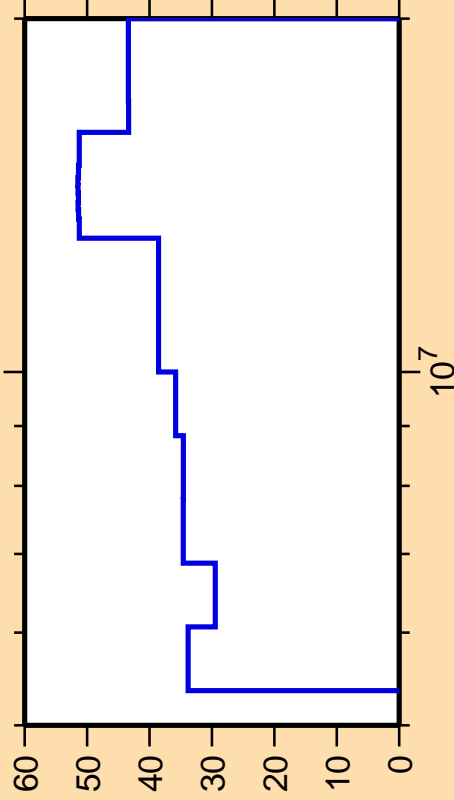
\Delta\sigma/\sigma vs. E for ^{168}\text{Ho}(n,\gamma)
