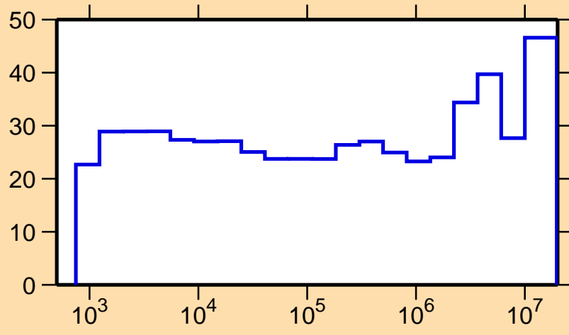
\Delta\sigma/\sigma vs. E for ^{168}\text{Ho}(n,\gamma)
