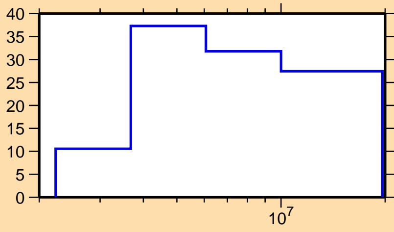
\Delta\sigma/\sigma vs. E for ^{168}\text{Ho}(n,p)
