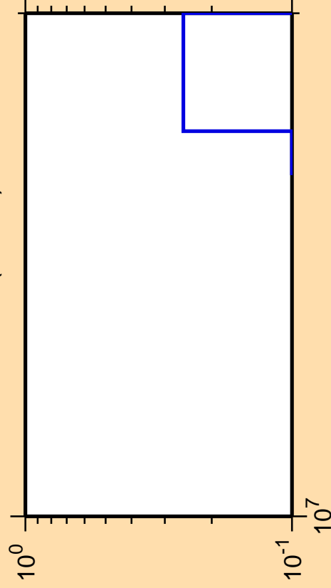
\Delta\sigma/\sigma vs. E for ^{168}\text{Ho}(n,3n\alpha)
