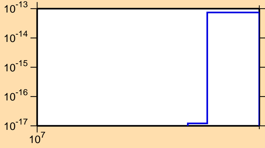
\sigma vs. E for ^{168}\text{Ho}(n,3n\alpha)
