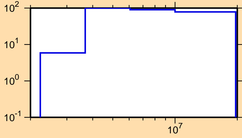
\Delta\sigma/\sigma vs. E for ^{168}\text{Ho}(n,p)
