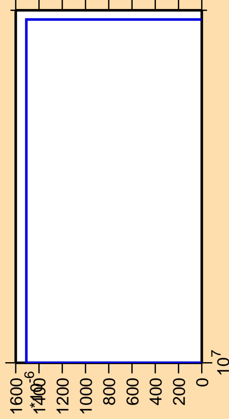
\Delta\sigma/\sigma vs. E for ^{168}\text{Ho}(n,3n\alpha)
