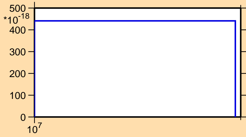
\sigma vs. E for ^{168}\text{Ho}(n,3n\alpha)
