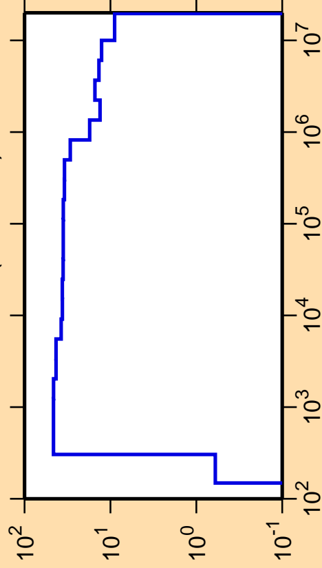
\Delta\sigma/\sigma vs. E for ^{168}\text{Ho}(n,\text{nonel.})
