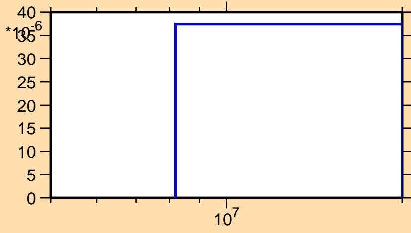
\sigma vs. E for ^{168}\text{Ho}(n,t)
