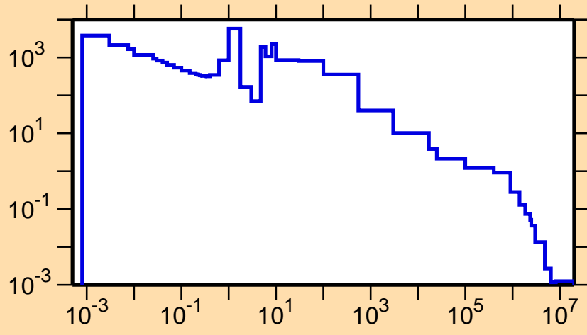
\sigma vs. E for ^{168}\text{Ho}(n,\gamma)
