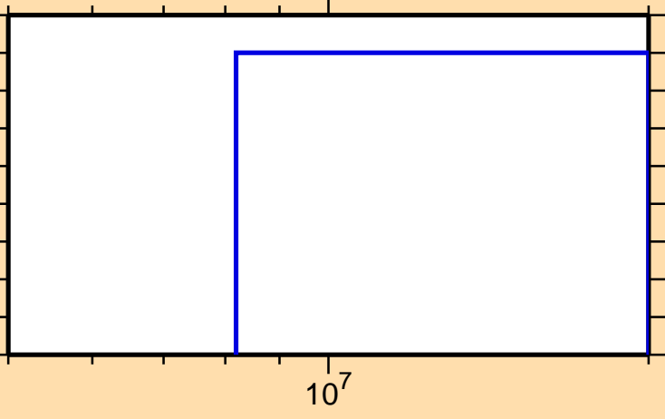
\sigma vs. E for ^{168}\text{Ho}(n,nt)
