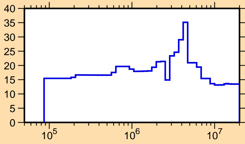
\Delta\sigma/\sigma vs. E for ^{169}\text{Ho}(n,n_1)
