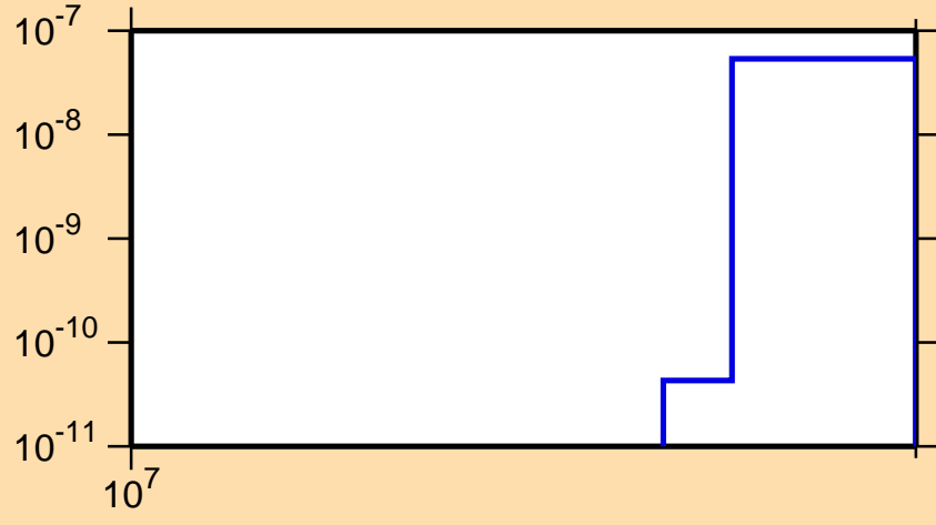
\sigma vs. E for ^{169}\text{Ho}(n,2np)
