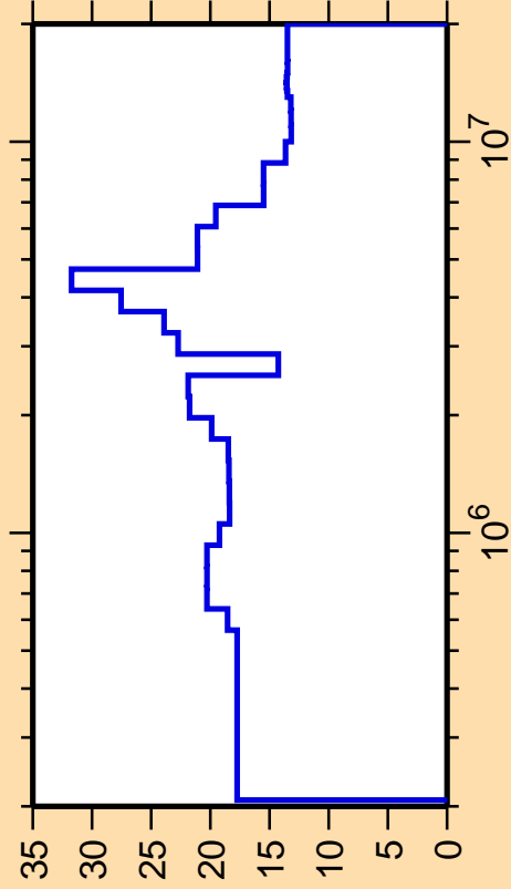
\Delta\sigma/\sigma vs. E for ^{169}\text{Ho}(n,n_2)
