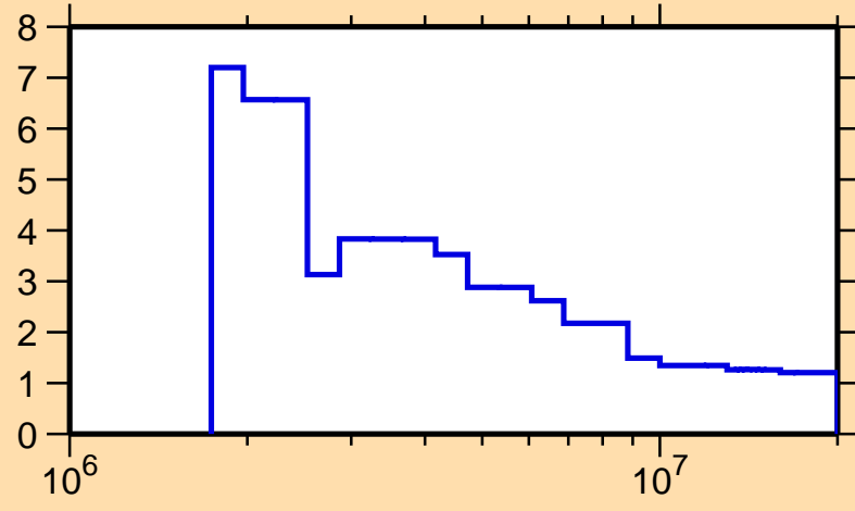
\Delta\sigma/\sigma vs. E for ^{169}\text{Ho}(n,n\text{onel.})
