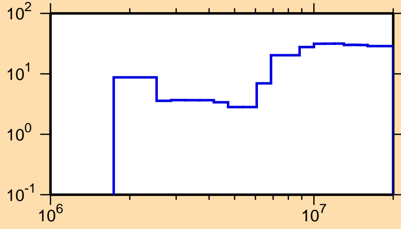
\Delta\sigma/\sigma vs. E for ^{169}\text{Ho}(n,n\text{cont.})
