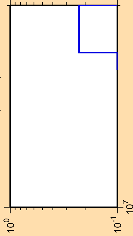
\Delta\sigma/\sigma vs. E for ^{169}\text{Ho}(n,3n\alpha)
