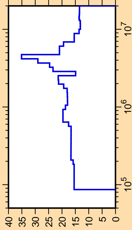
\Delta\sigma/\sigma vs. E for ^{169}\text{Ho}(n,n_1)
