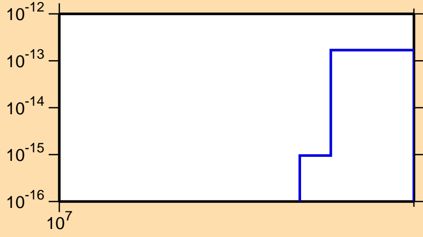
\sigma vs. E for ^{169}\text{Ho}(n,3n\alpha)
