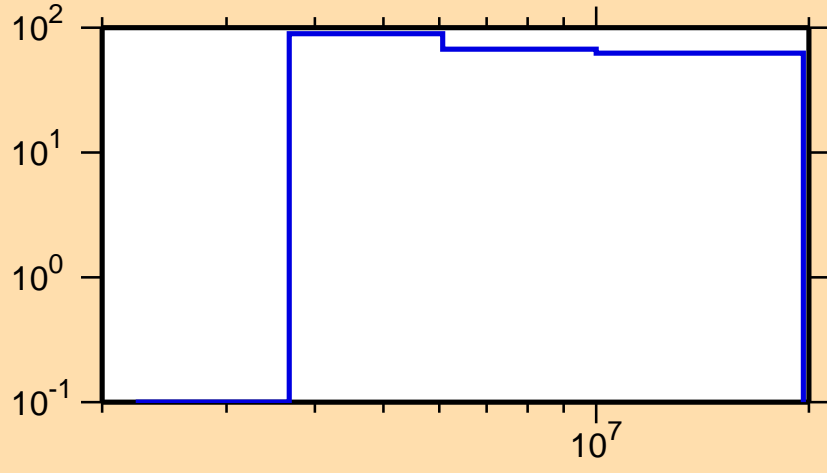
\Delta\sigma/\sigma vs. E for ^{170}\text{Ho}(n,p)
