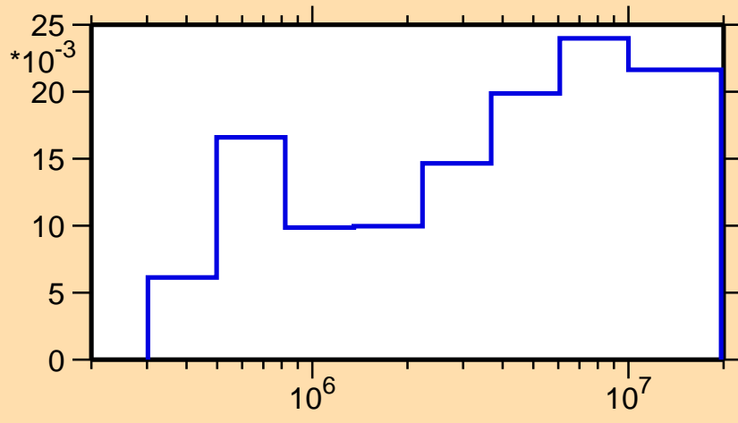
\sigma vs. E for ^{170}\text{Ho}(n,n_4)
