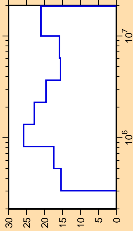
\Delta\sigma/\sigma vs. E for ^{170}\text{Ho}(n,n_4)
