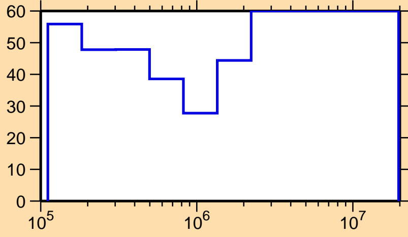
\Delta\sigma/\sigma vs. E for ^{170}\text{Ho}(n,n_1)
