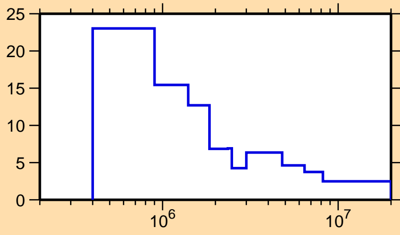
\Delta\sigma/\sigma vs. E for ^{170}\text{Ho}(n,n\text{onel.})
