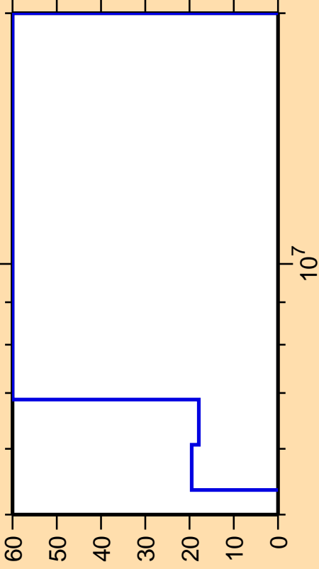
\Delta\sigma/\sigma vs. E for ^{170}\text{Ho}(n,n\text{cont.})
