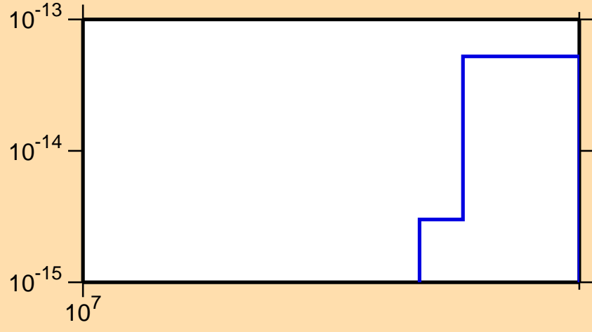
\sigma vs. E for ^{170}\text{Ho}(n,3n\alpha)
