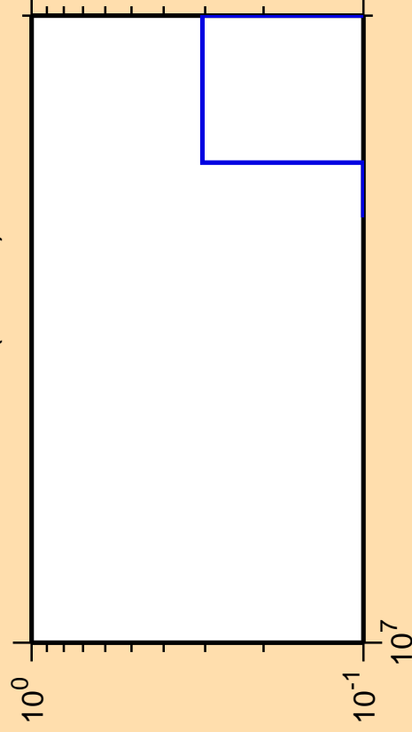
\Delta\sigma/\sigma vs. E for ^{170}\text{Ho}(n,3n\alpha)
