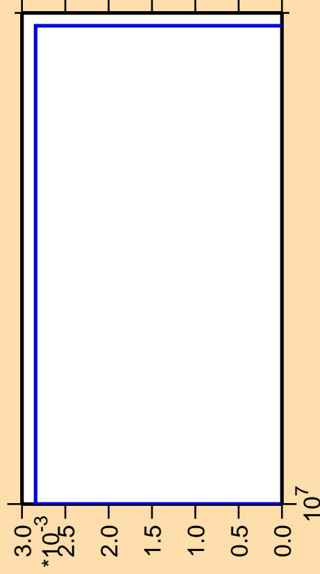
\Delta\sigma/\sigma vs. E for ^{170}\text{Ho}(n,3n\alpha)
