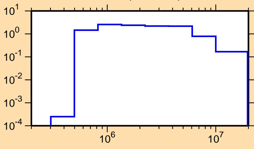
\sigma vs. E for ^{170}\text{Ho}(n,n\text{cont.})
