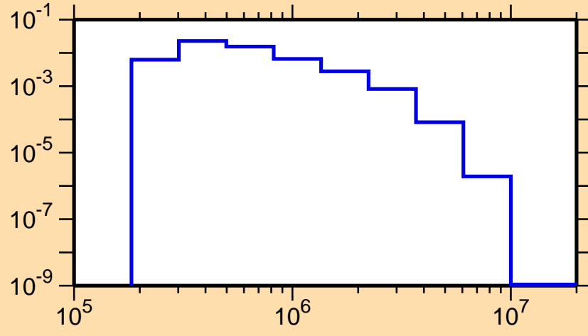
\sigma vs. E for ^{170}\text{Ho}(n,n_2)
