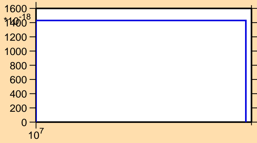
\sigma vs. E for ^{170}\text{Ho}(n,3n\alpha)
