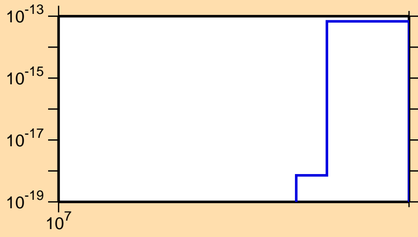
\sigma vs. E for ^{171}\text{Ho}(n,3n\alpha)
