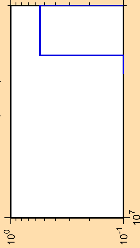
\Delta\sigma/\sigma vs. E for ^{171}\text{Ho}(n,3n\alpha)
