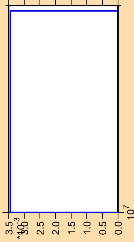
\Delta\sigma/\sigma vs. E for ^{171}\text{Ho}(n,3n\alpha)
