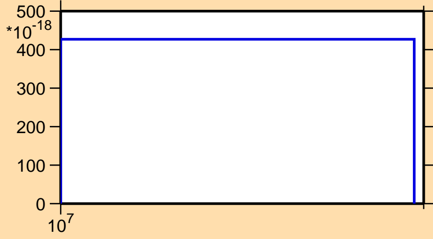
\sigma vs. E for ^{171}\text{Ho}(n,3n\alpha)
