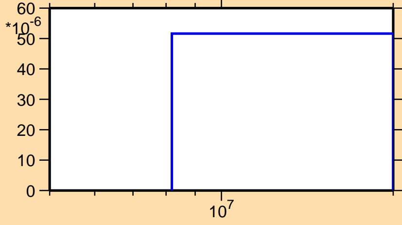
\sigma vs. E for ^{171}\text{Ho}(n,np)
