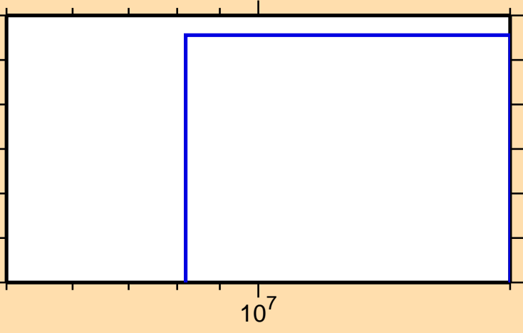
\sigma vs. E for ^{171}\text{Ho}(n,3n\alpha)
