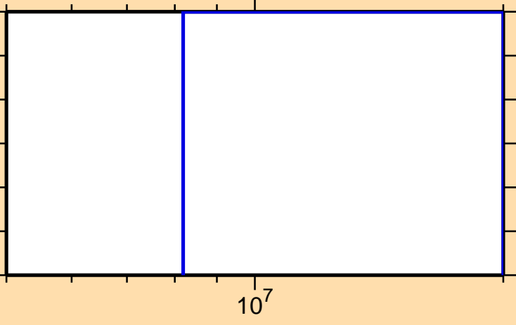
\sigma vs. E for ^{171}\text{Ho}(n,d)
