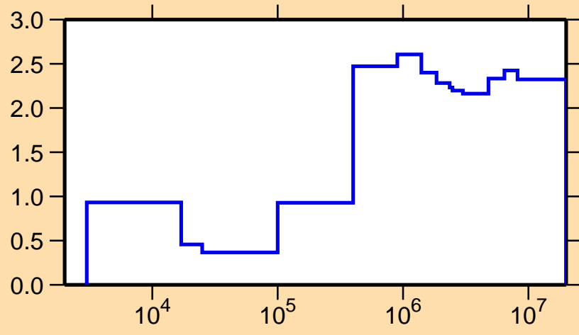
\sigma vs. E for ^{171}\text{Ho}(n,\text{nonel.})
