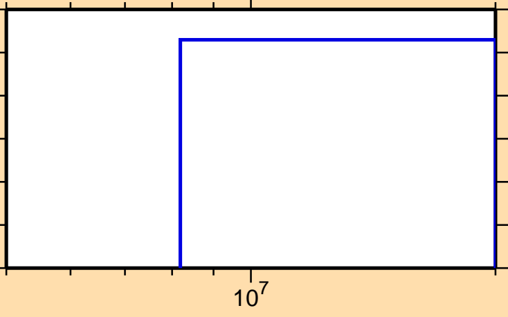
\sigma vs. E for ^{171}\text{Ho}(n,2np)
