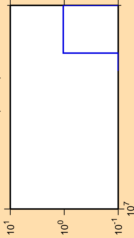
\Delta\sigma/\sigma vs. E for ^{172}\text{Ho}(n,3n\alpha)
