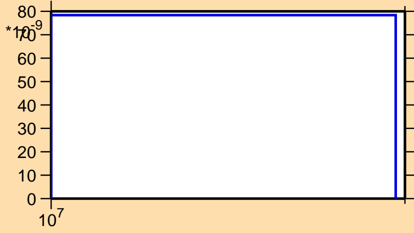
\sigma vs. E for ^{172}\text{Ho}(n,\text{nd})
