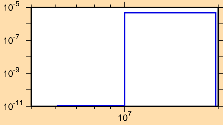
\sigma vs. E for ^{172}\text{Ho}(n,n\alpha)
