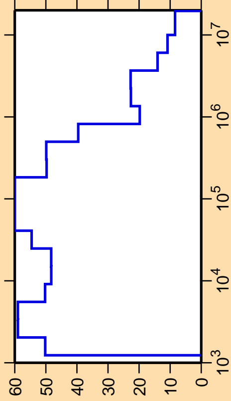
\Delta\sigma/\sigma vs. E for ^{172}\text{Ho}(n,\text{nonel.})
