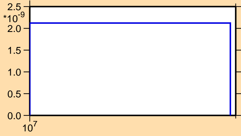
\sigma vs. E for ^{172}\text{Ho}(n,2n\alpha)
