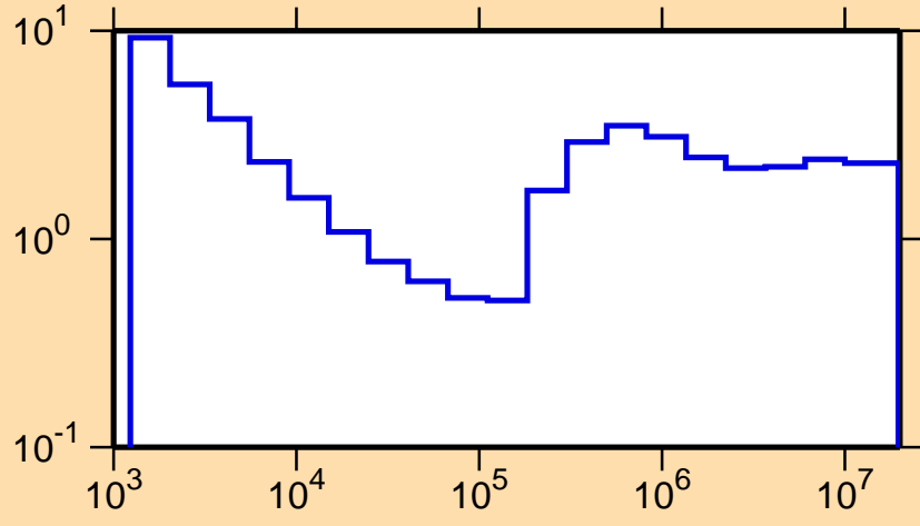
\sigma vs. E for ^{172}\text{Ho}(n,\text{nonel.})
