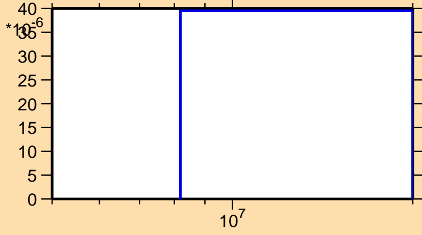
\sigma vs. E for ^{172}\text{Ho}(n,np)
