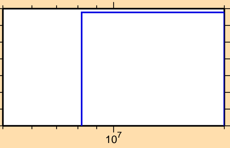
\sigma vs. E for ^{172}\text{Ho}(n,\text{nd})
