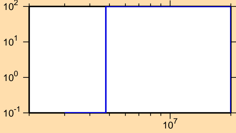
\Delta\sigma/\sigma vs. E for ^{172}\text{Ho}(n,p)
