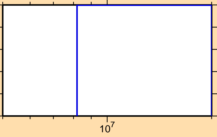
\sigma vs. E for ^{172}\text{Ho}(n,d)
