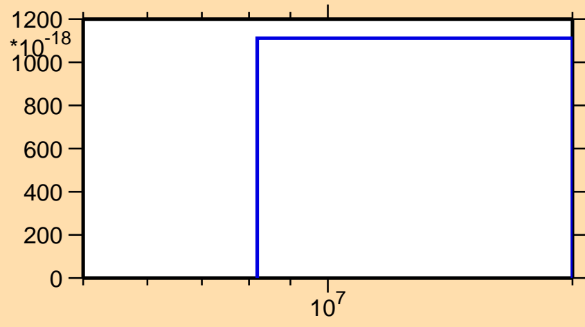
\sigma vs. E for ^{172}\text{Ho}(n,3n\alpha)
