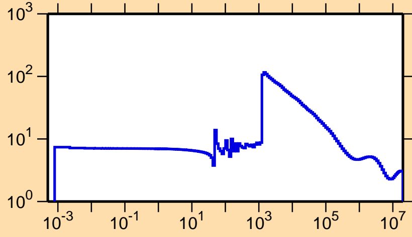
\sigma vs. E for ^{173}\text{Ho}(n,\text{el.})
