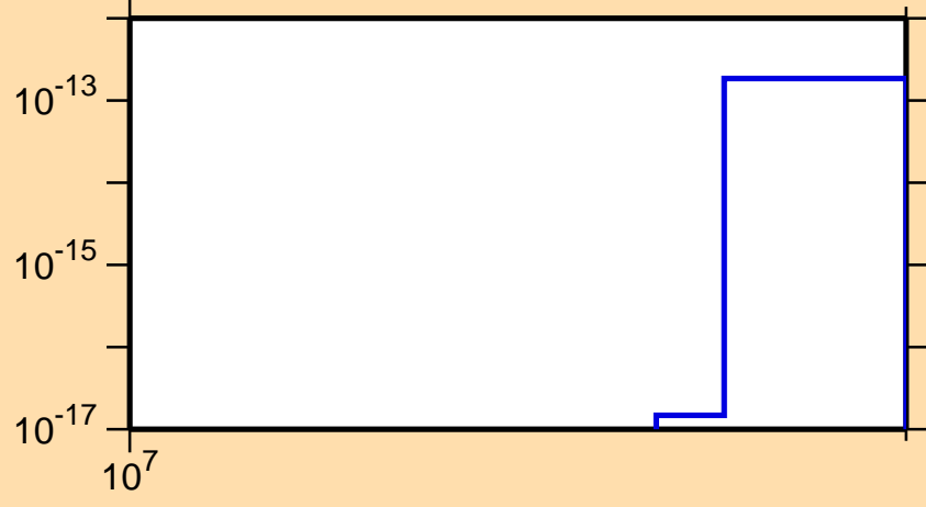
\sigma vs. E for ^{173}\text{Ho}(n,3n\alpha)
