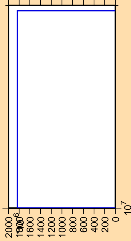
\Delta\sigma/\sigma vs. E for ^{173}\text{Ho}(n,3n\alpha)
