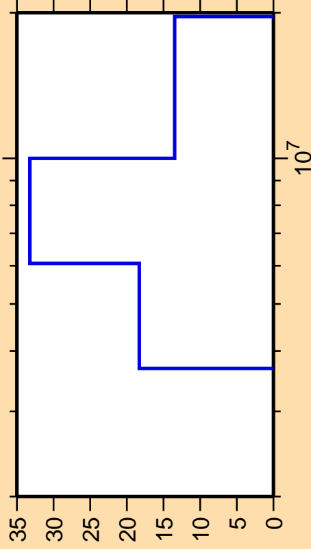
\Delta\sigma/\sigma vs. E for ^{173}\text{Ho}(n,n\text{cont.})
