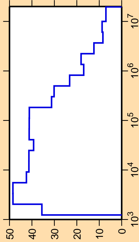
\Delta\sigma/\sigma vs. E for ^{173}\text{Ho}(n,\text{nonel.})
