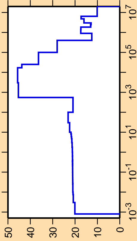
\Delta\sigma/\sigma vs. E for ^{173}\text{Ho}(n,\text{el.})
