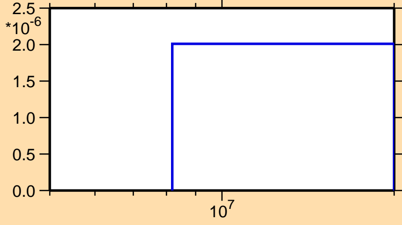
\sigma vs. E for ^{173}\text{Ho}(n,n\alpha)
