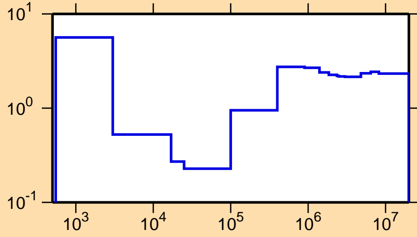
\sigma vs. E for ^{173}\text{Ho}(n,\text{nonel.})
