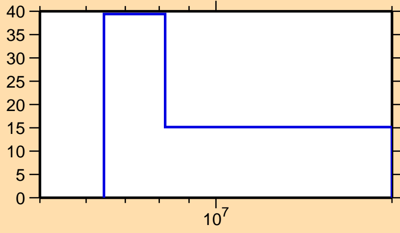
\Delta\sigma/\sigma vs. E for ^{173}\text{Ho}(n,ncont.)
