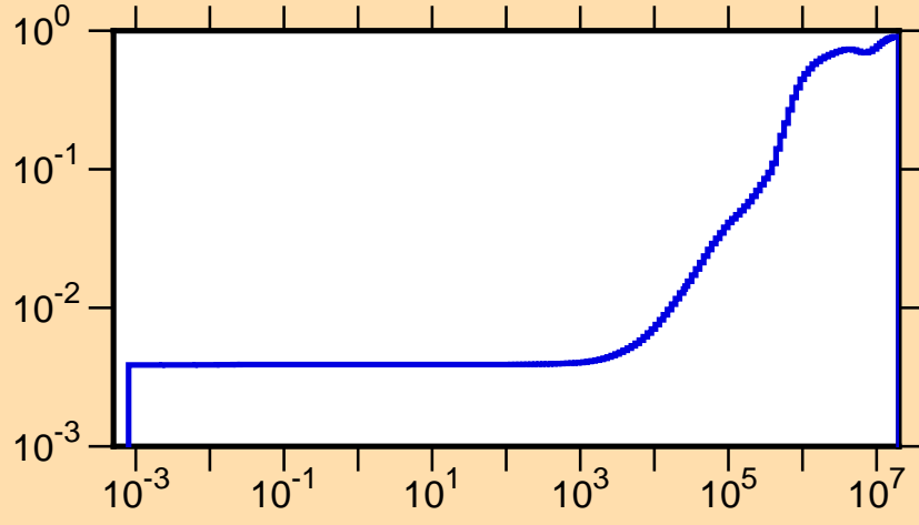
\mu vs. E for ^{174}\text{Ho}(\text{mt251})
