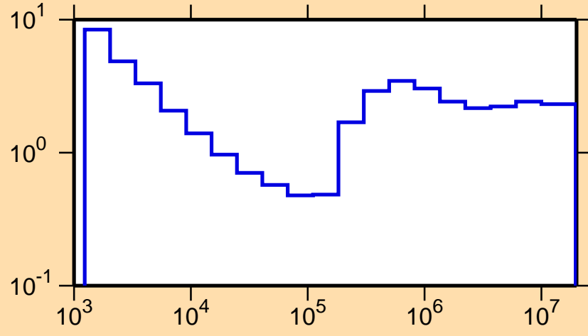
\sigma vs. E for ^{174}\text{Ho}(n,\text{nonel.})
