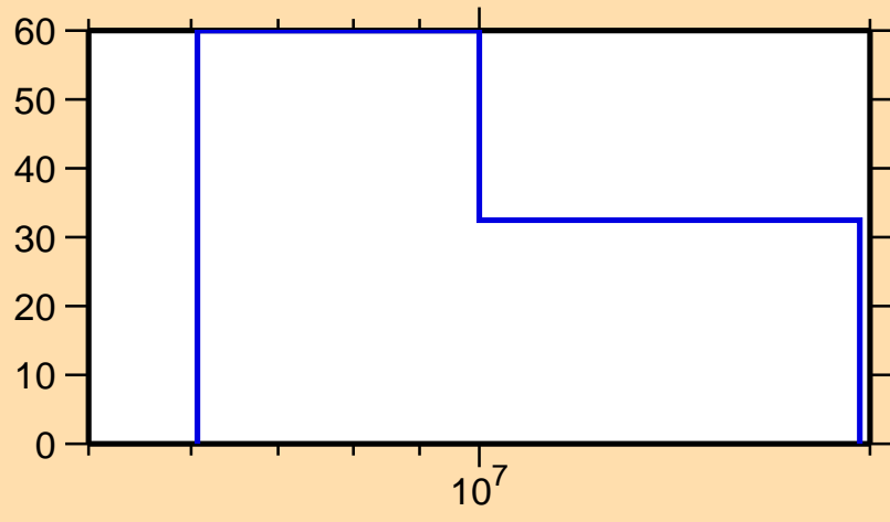
\Delta\sigma/\sigma vs. E for ^{174}\text{Ho}(n,ncont.)
