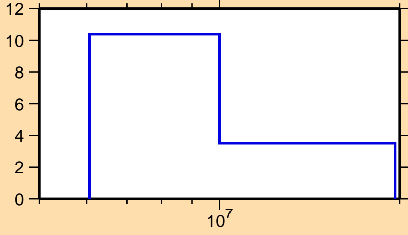
\Delta\sigma/\sigma vs. E for ^{174}\text{Ho}(n,el.)
