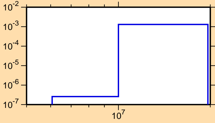
\sigma vs. E for ^{174}\text{Ho}(n,p)
